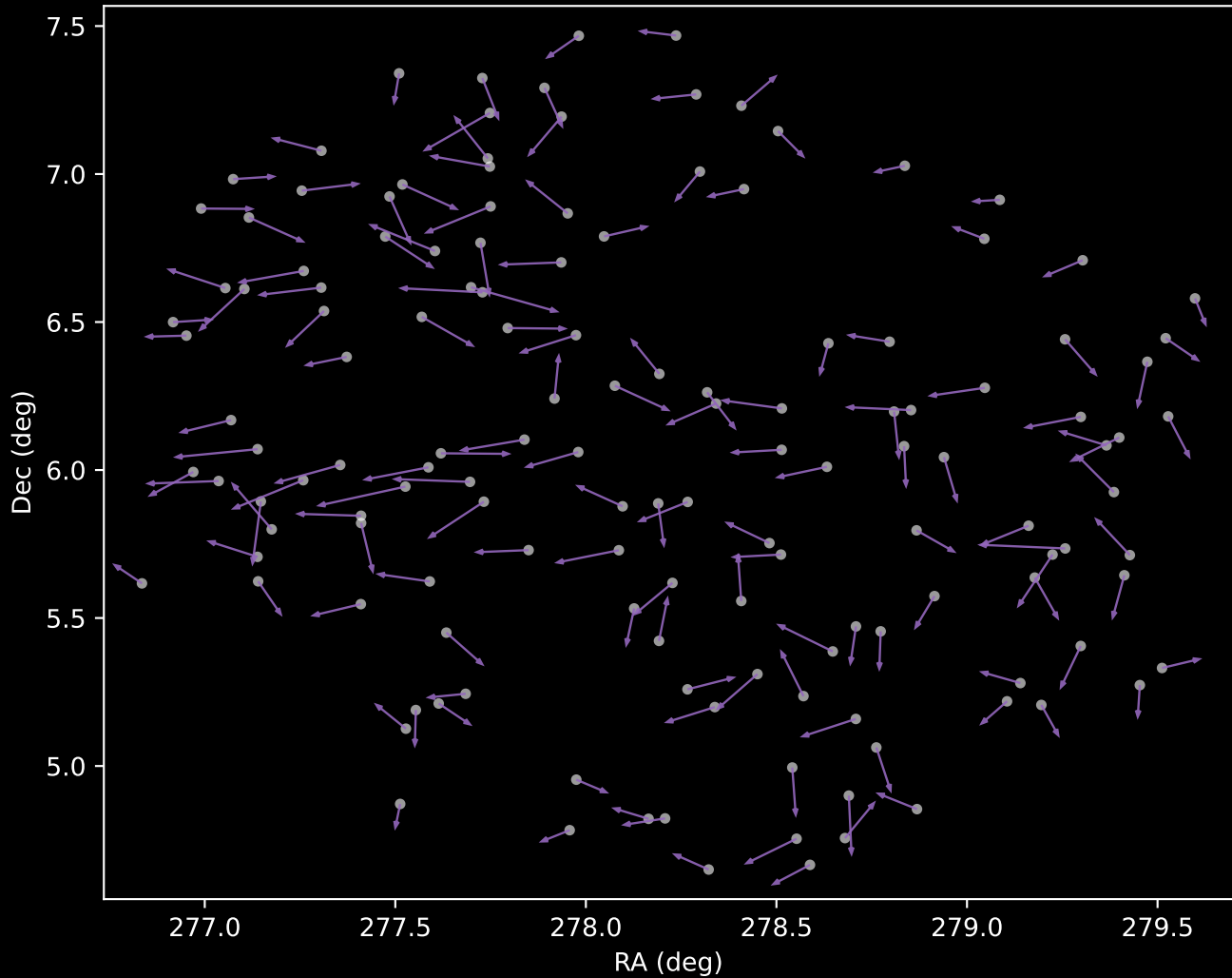
APOGEE DR17 Cluster 8 Proper Motion Vectors (n=142)
