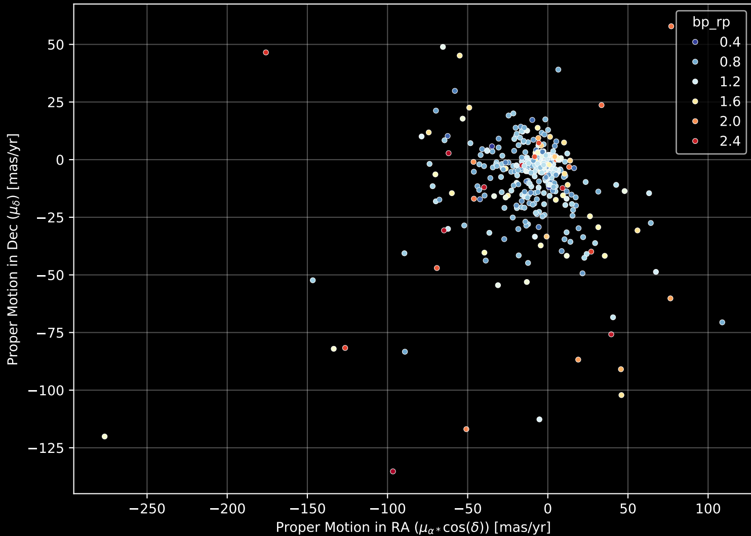
APOGEE DR17 Field: [266+64_btx] Proper Motion Diagram (n= 344)
