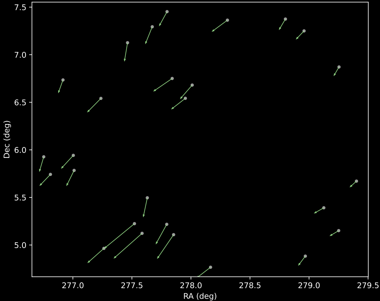
APOGEE DR17 Cluster 5 Proper Motion Vectors (n=27)
