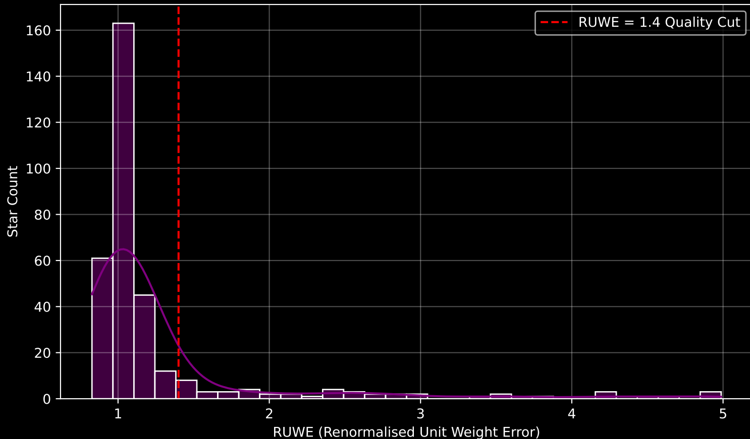
GAPOGEE DR17 Field [266+64_btx] RUWE Distribution (n= 330)
