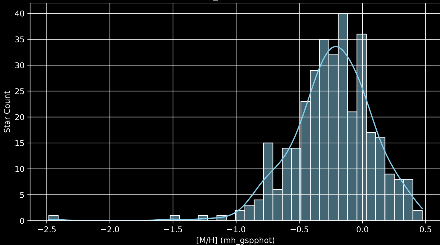
APOGEE DR17 Field: [266+64_btx [M/H] (mh_gspphot) (n= 338)
