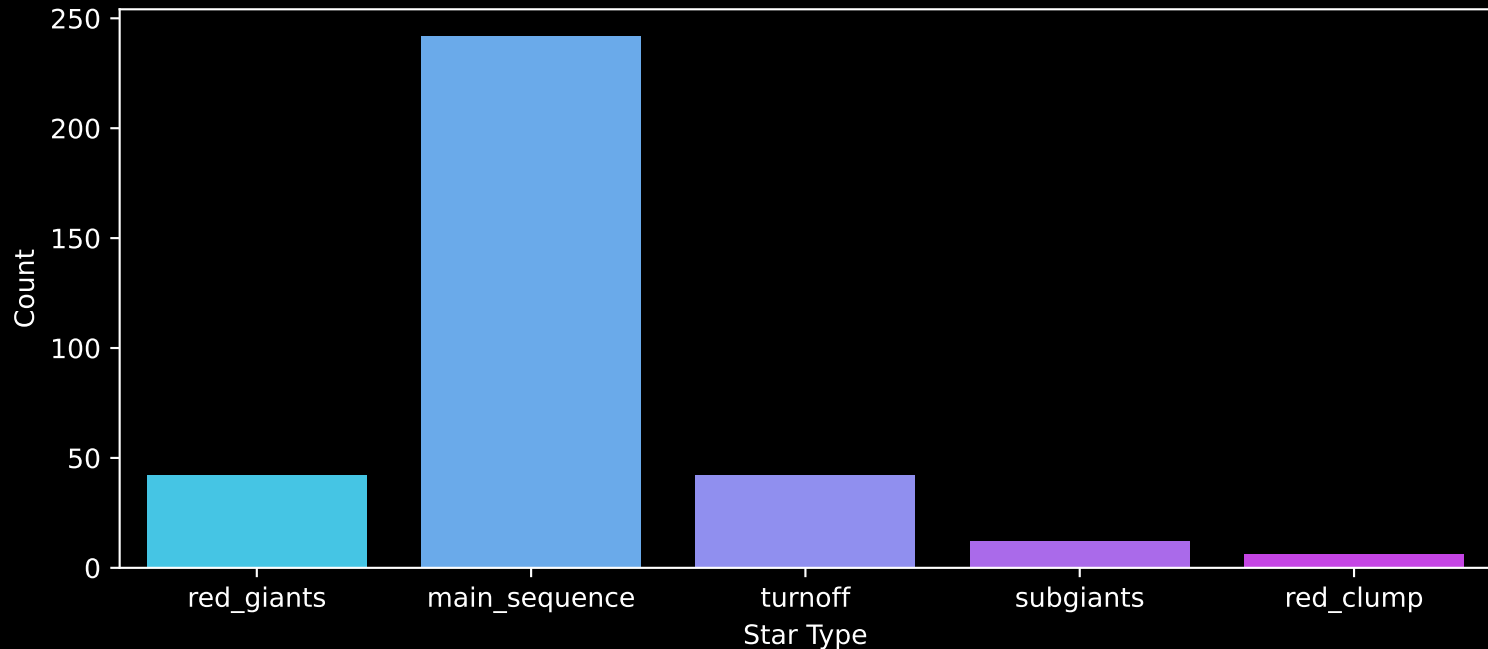
APOGEE DR17 Field: [266+64_btx] Count plot of Star Type
