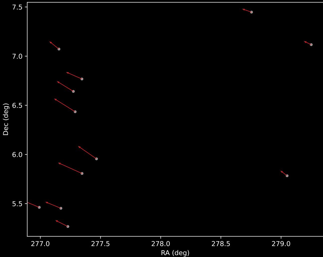
APOGEE DR17 Cluster 6 Proper Motion Vectors (n=12)
