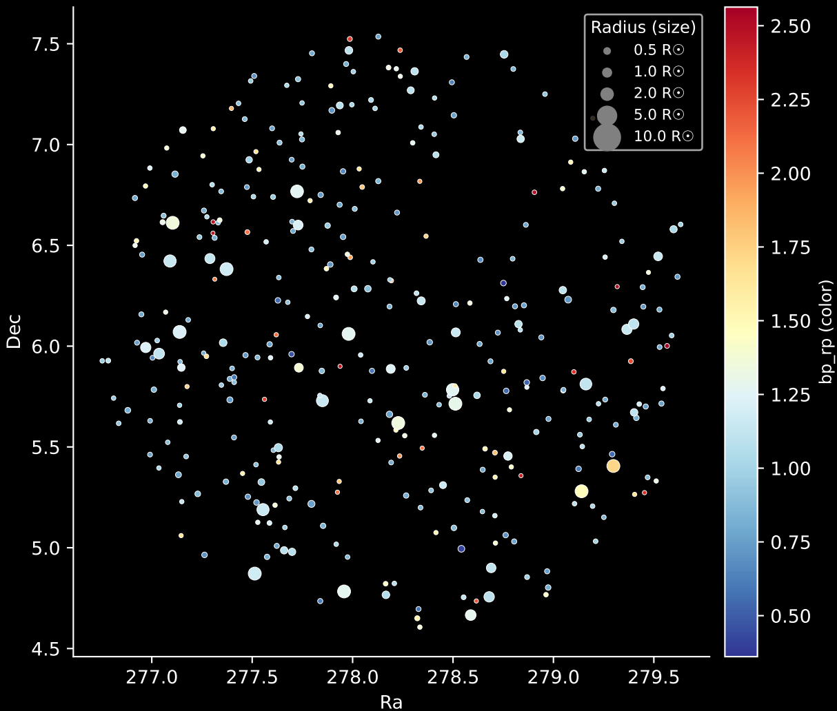
APOGEE DR17 Field: [266+64_btx] Stars: 344
