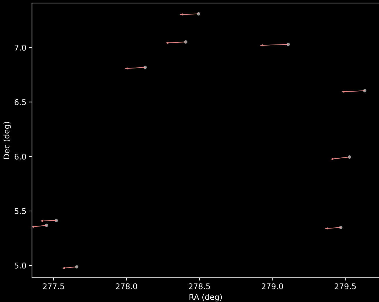
APOGEE DR17 Cluster 7 Proper Motion Vectors (n=10)
