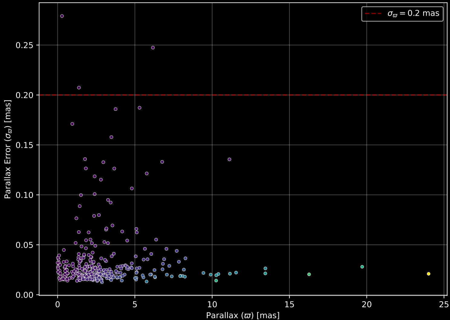
APOGEE DR17 Field: [266+64_btx] Parallax Quality (n= 344)
